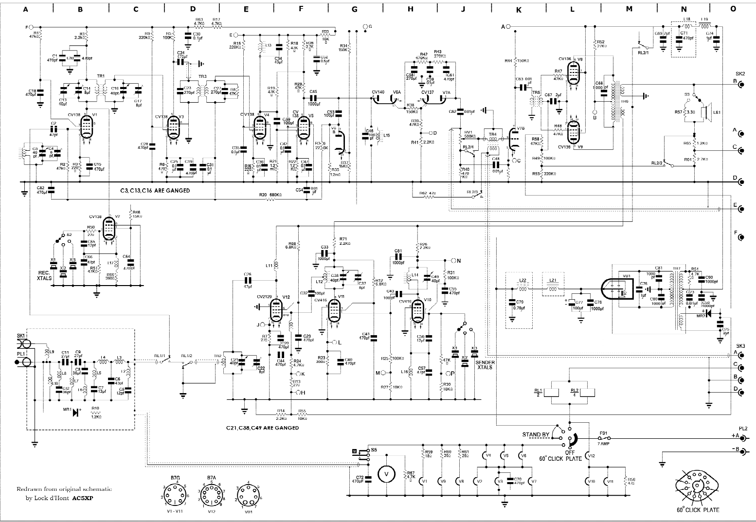
- Circuit diagram WS-B44 Mk3
