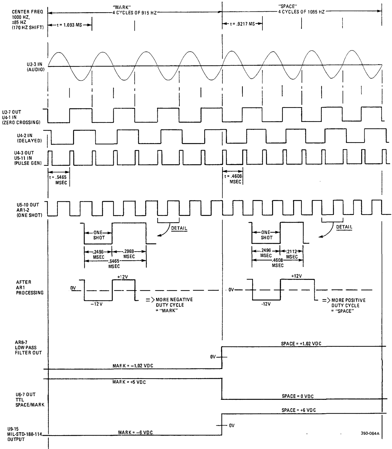
Figure 5-32. AFSK Converter Timing Diagram
