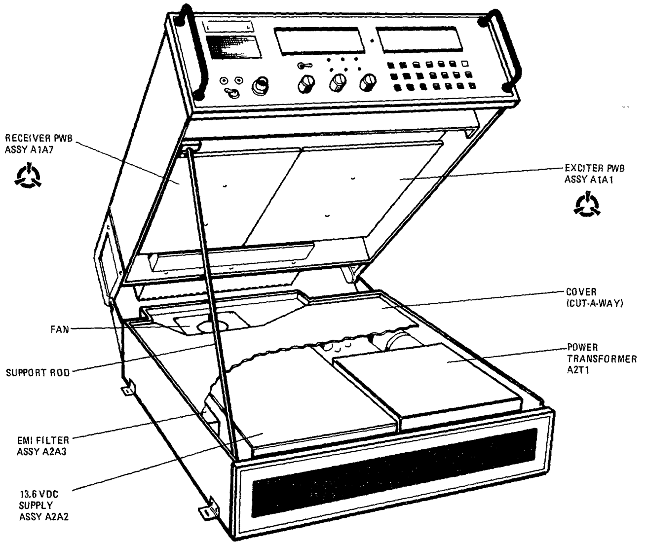
C. TRANSCIEVER ASSEMBLY UNLATCHED AND RAISED
