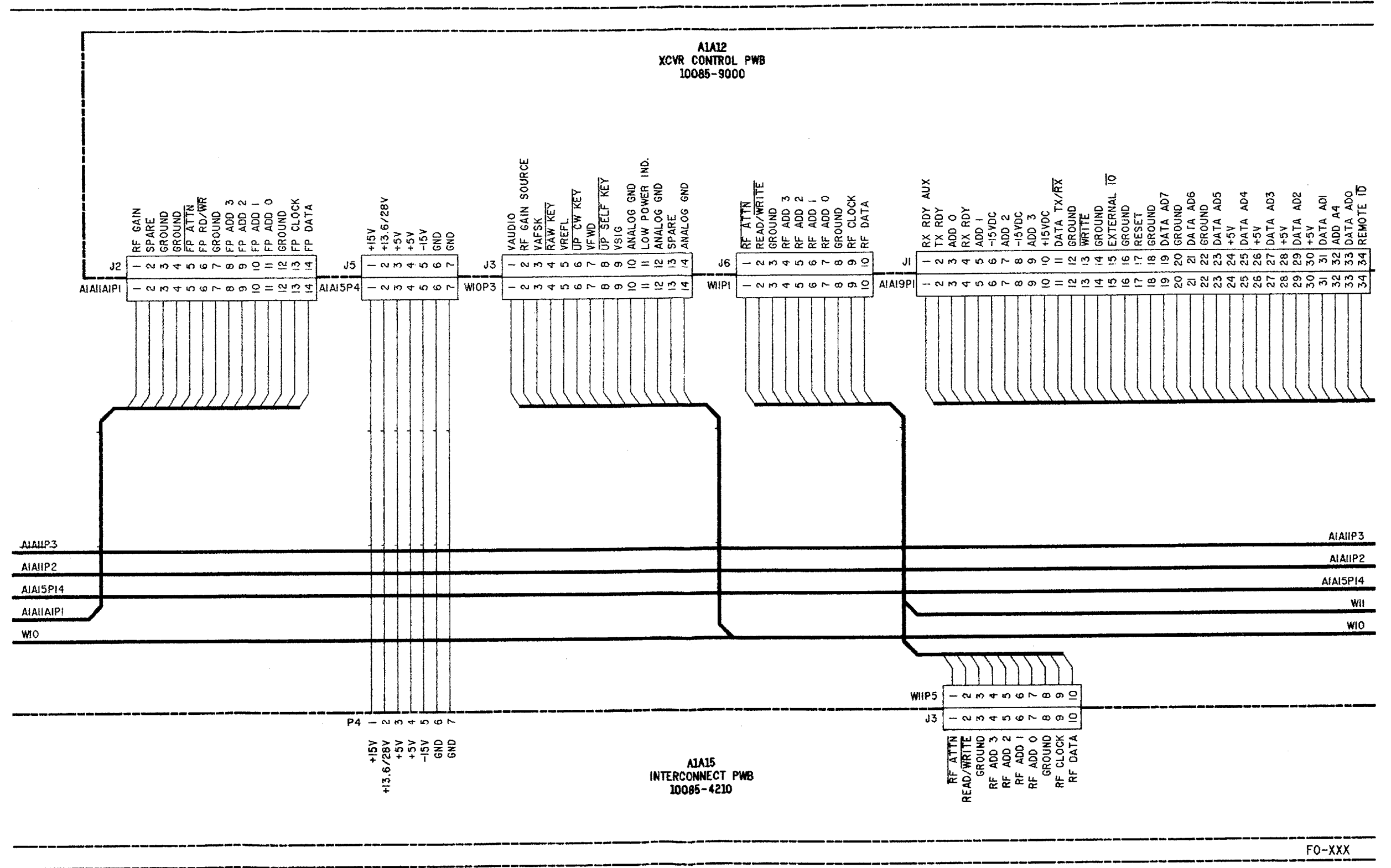
Figure FO-11. Interconnection Diagram. (Sheet 2 of 13)
