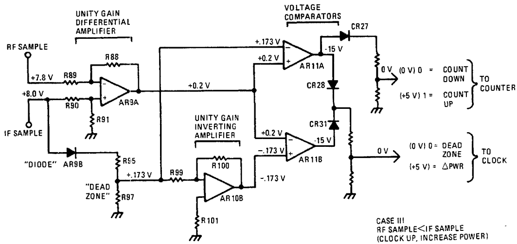
Figure 5-8. Simplified TGC Detector Operation
