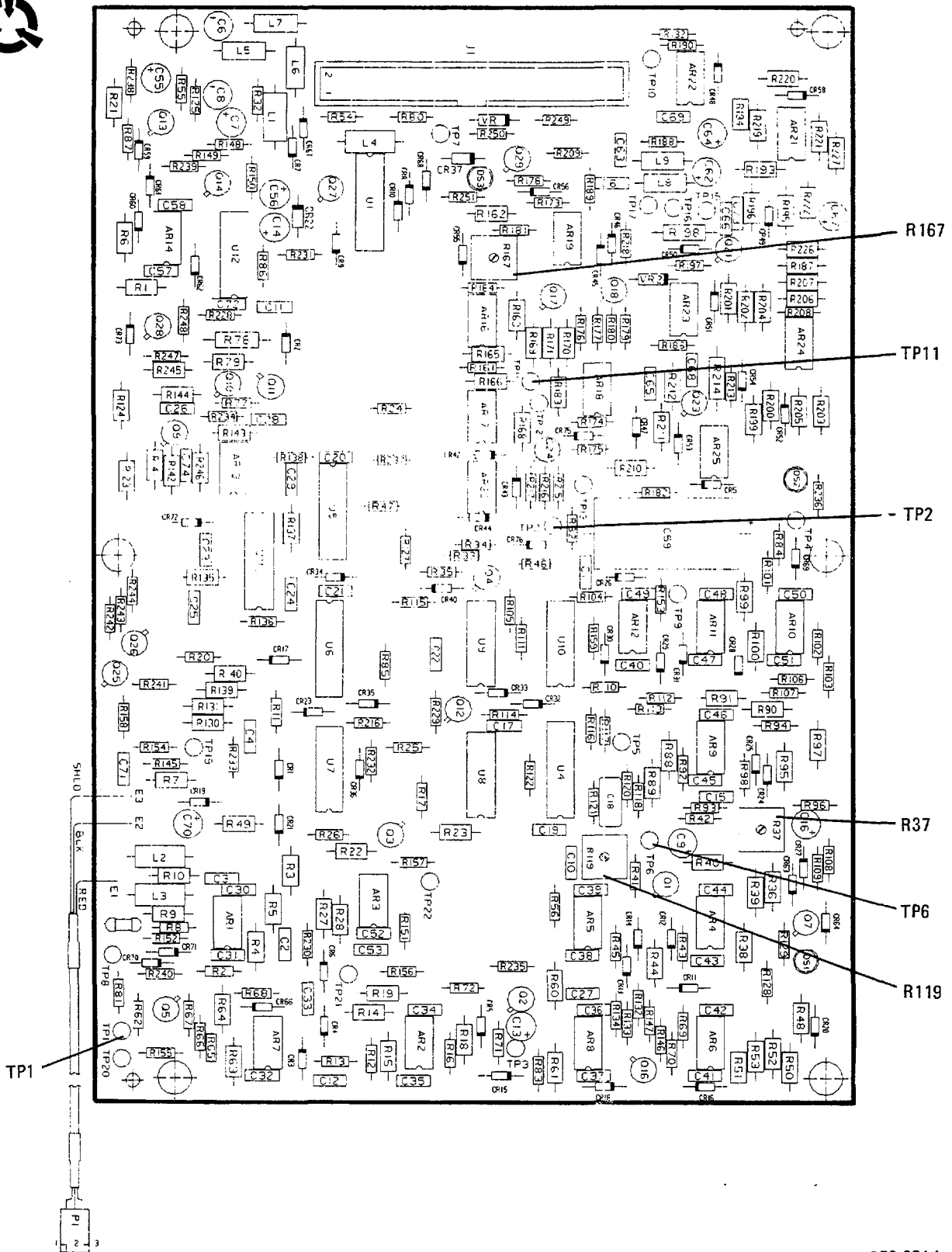
Figure 6-8. AGC/TGC PWB Assy.
