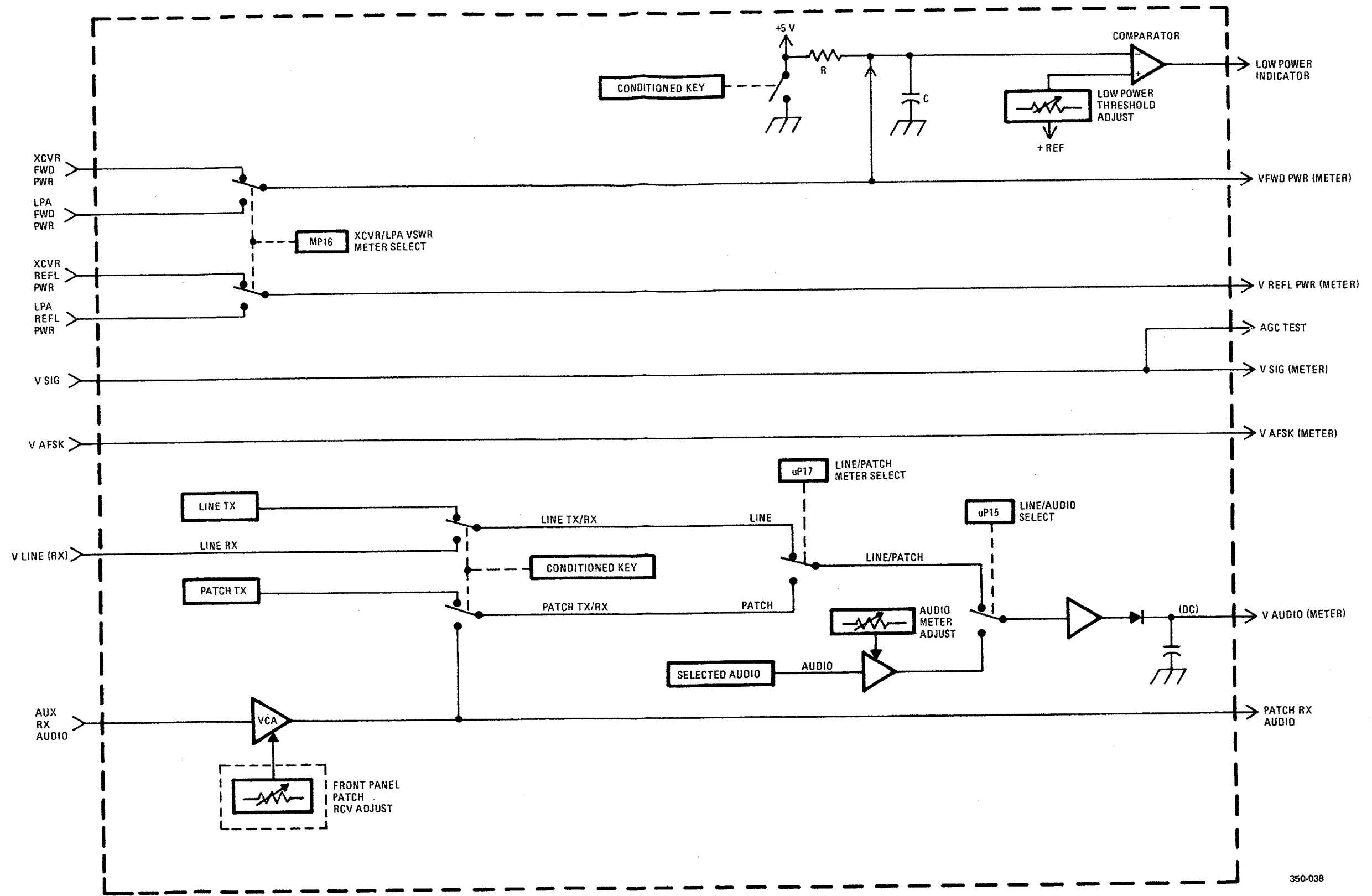
Figure FO-5. Simplified Exciter Meter Select Path.
