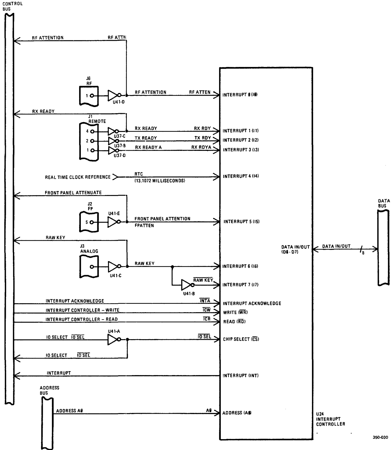
Figure 5-24. Simplified Interrupt Controller Circuits
