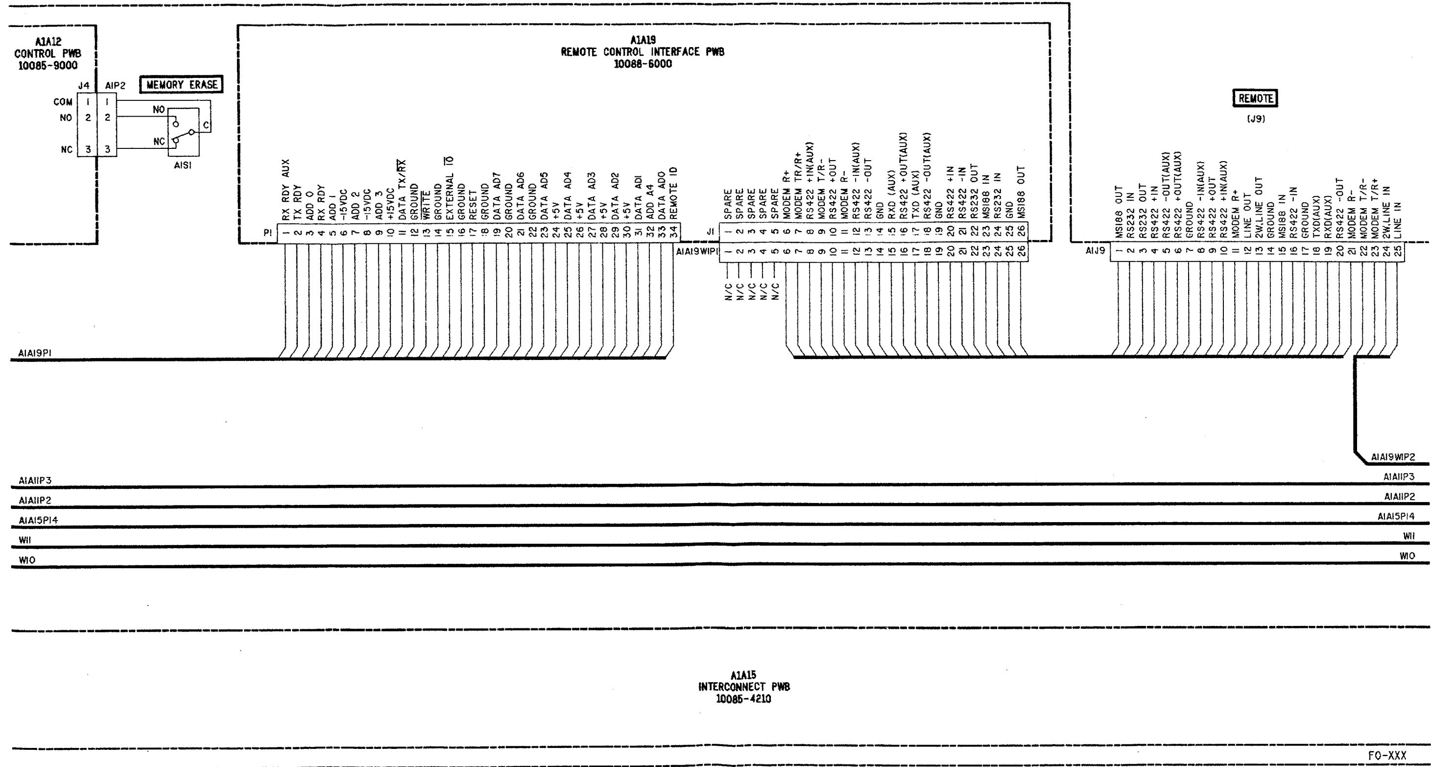
Figure FO-11. Interconnection Diagram. (Sheet 3 of 13)
