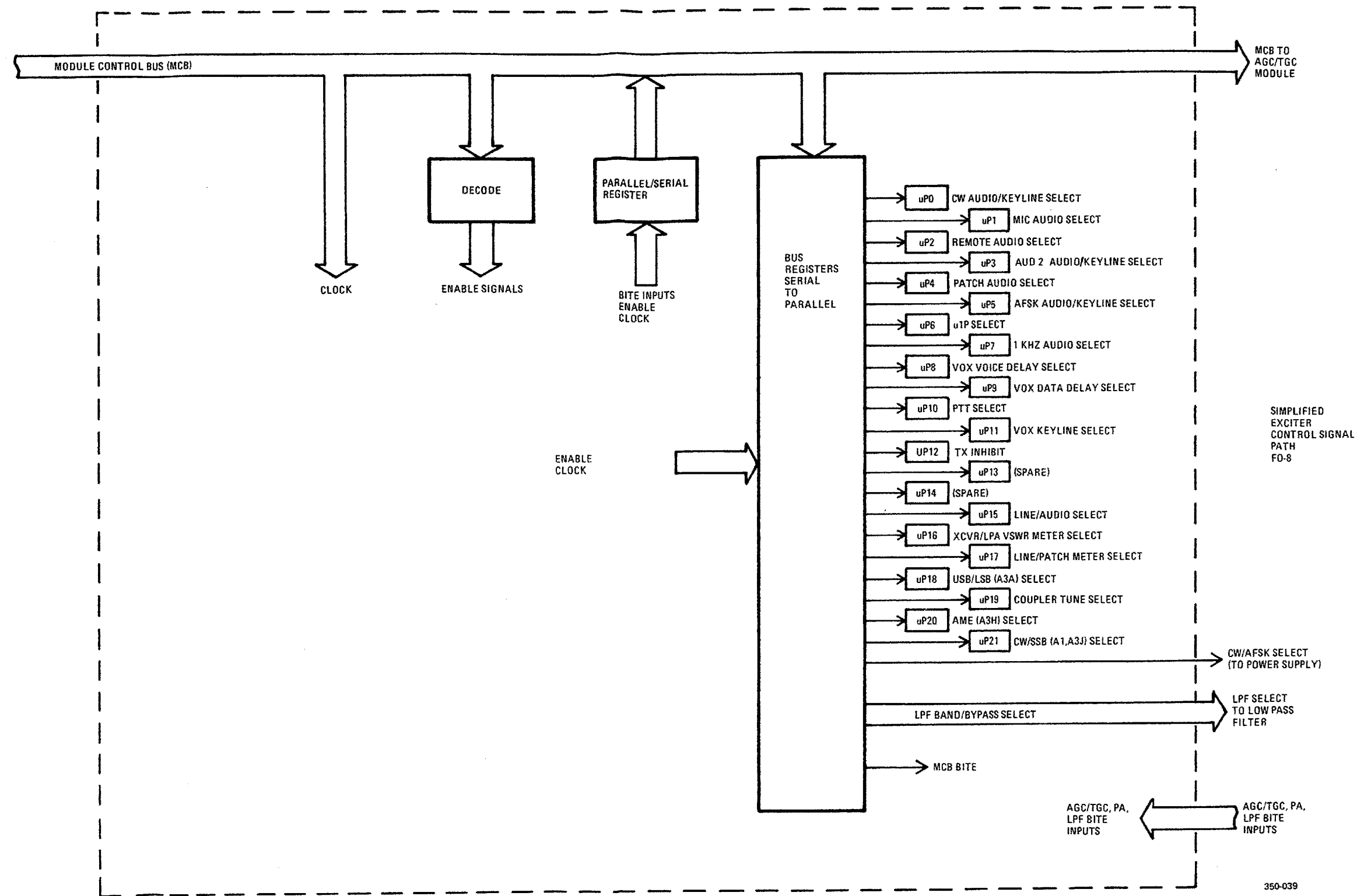
Figure FO-6. Simplified Exciter Control Signal Path.
