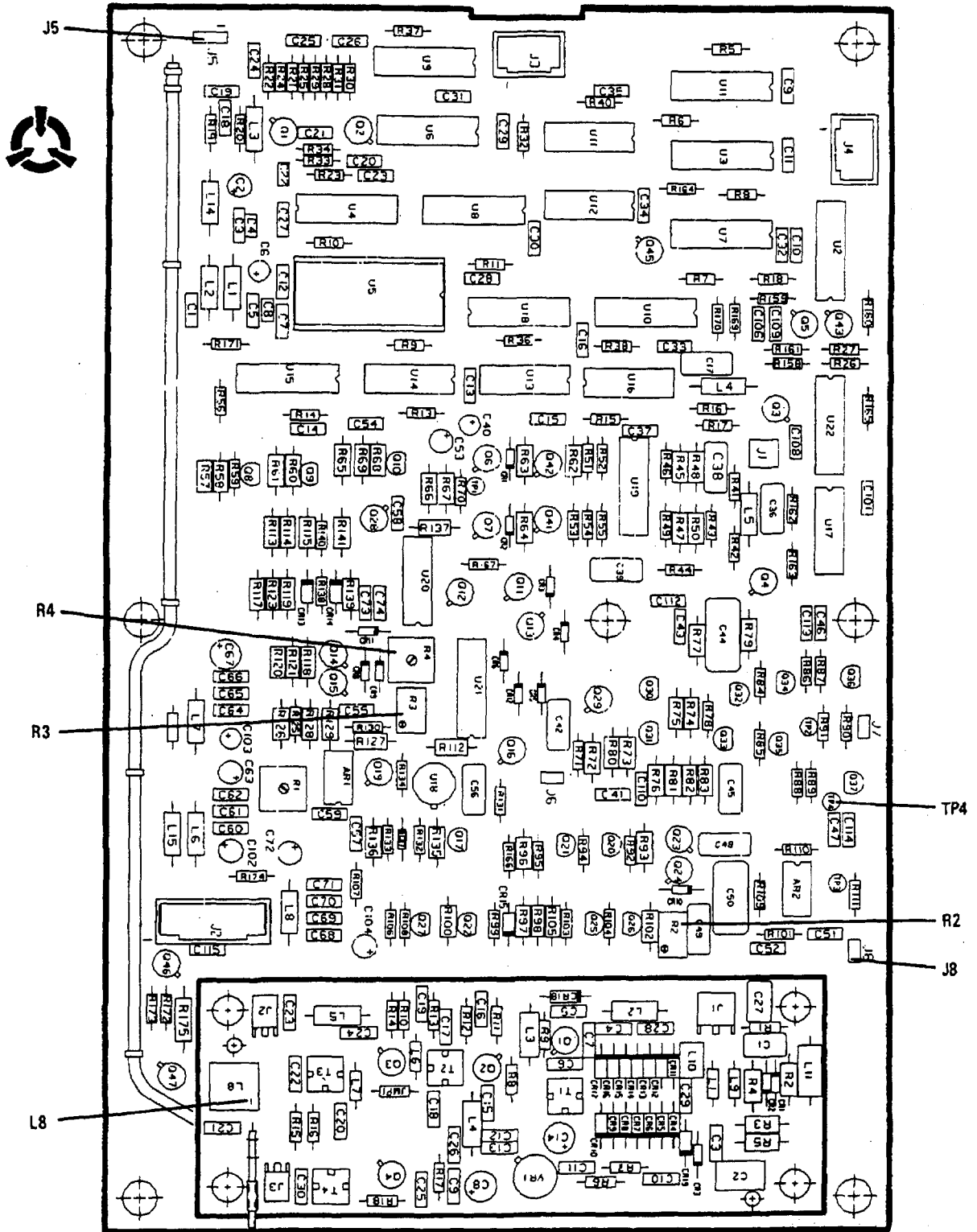
Figure 6-12. Synthesizer PWB Assy.
