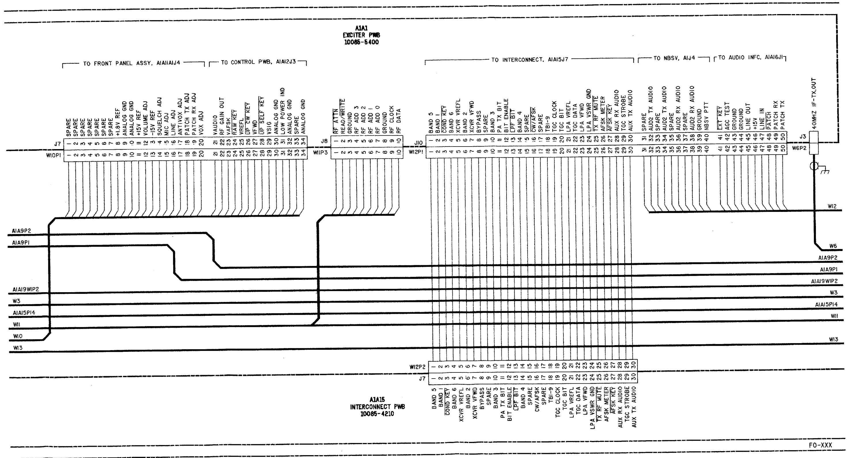
Figure FO-11. Interconnection Diagram. (Sheet 7 of 13)
