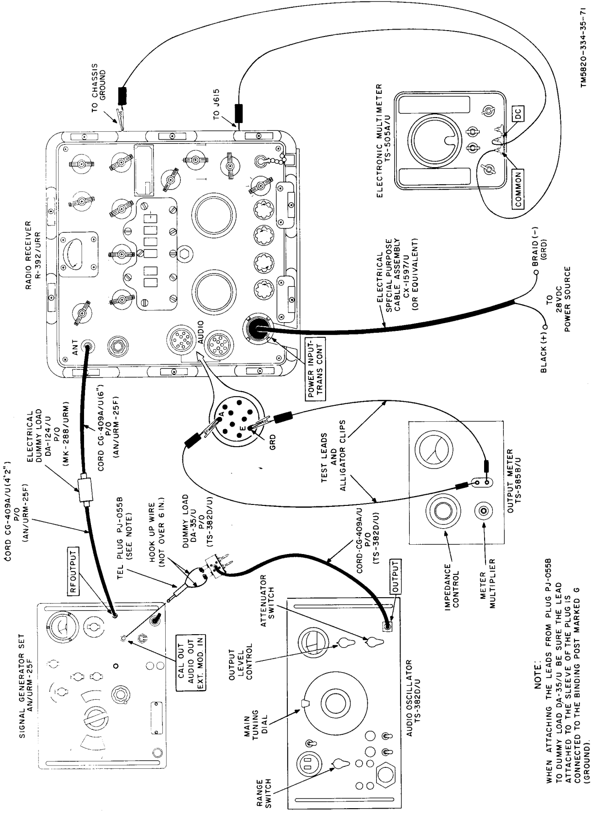
Figure 71. Overall audio response test.
