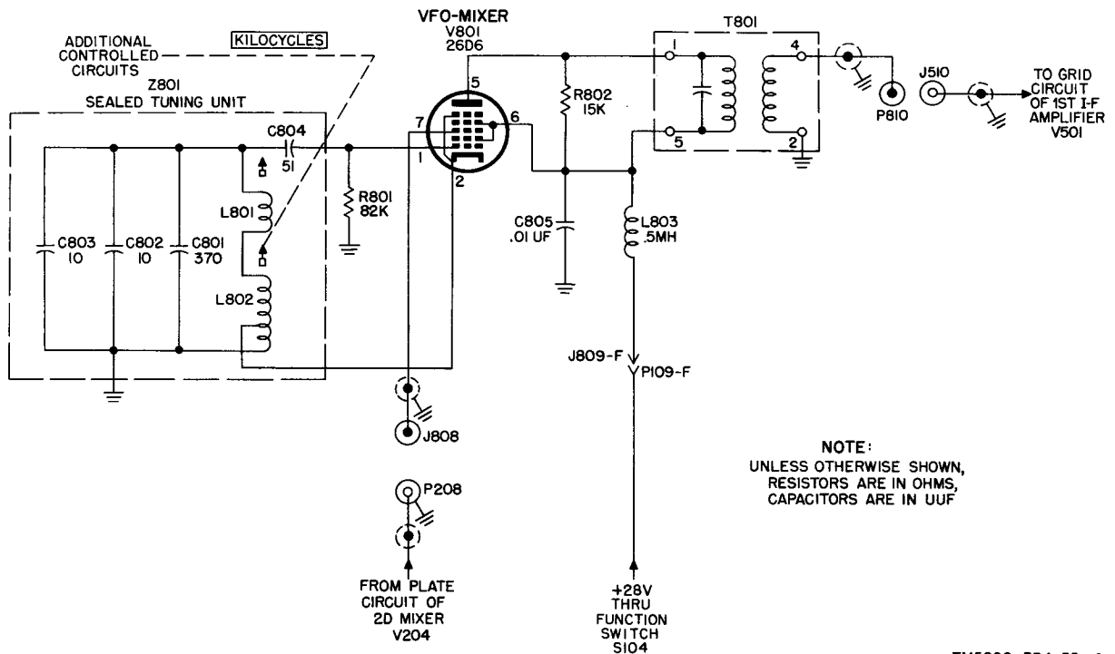
Figure 8. Vfo-mixer, simplified schematic diagram.
