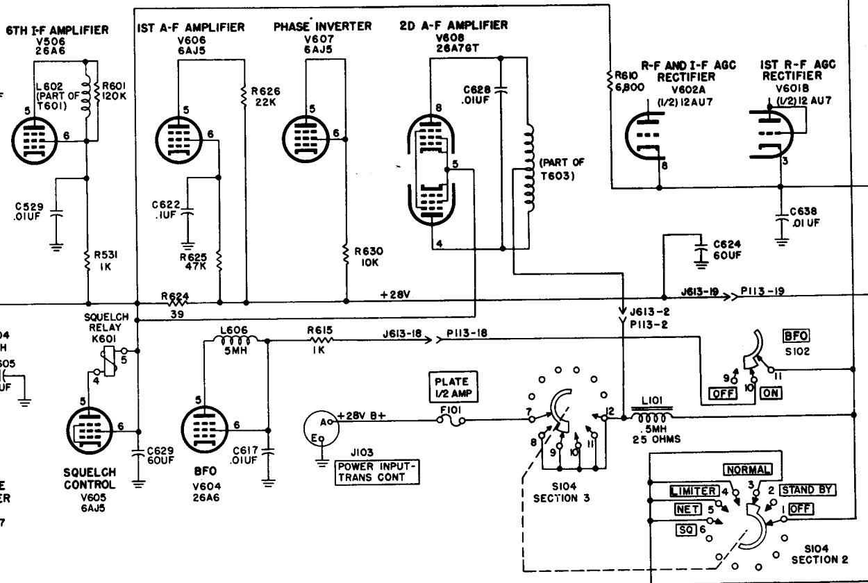
Plate and screen voltage distribution, schematic diagram.
