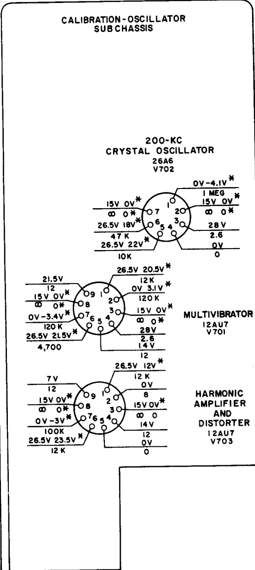
Voltage and resistance diagram.
