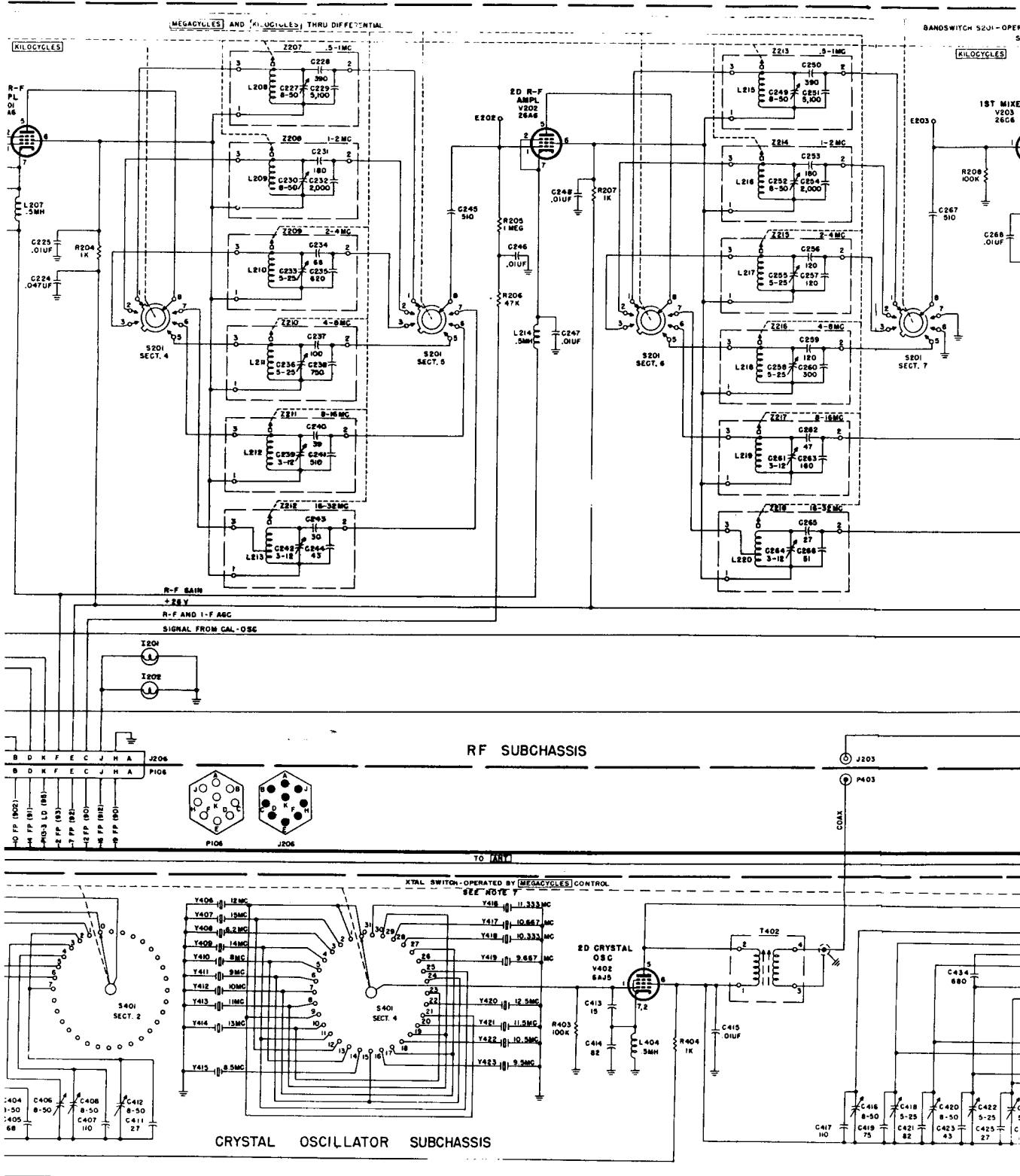
Figure 88(1). Radio receiver, wiring diagram (part 1 of 21).
