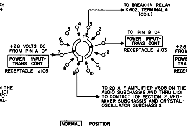
Figure 26. Function switch S104, schematic diagram.
