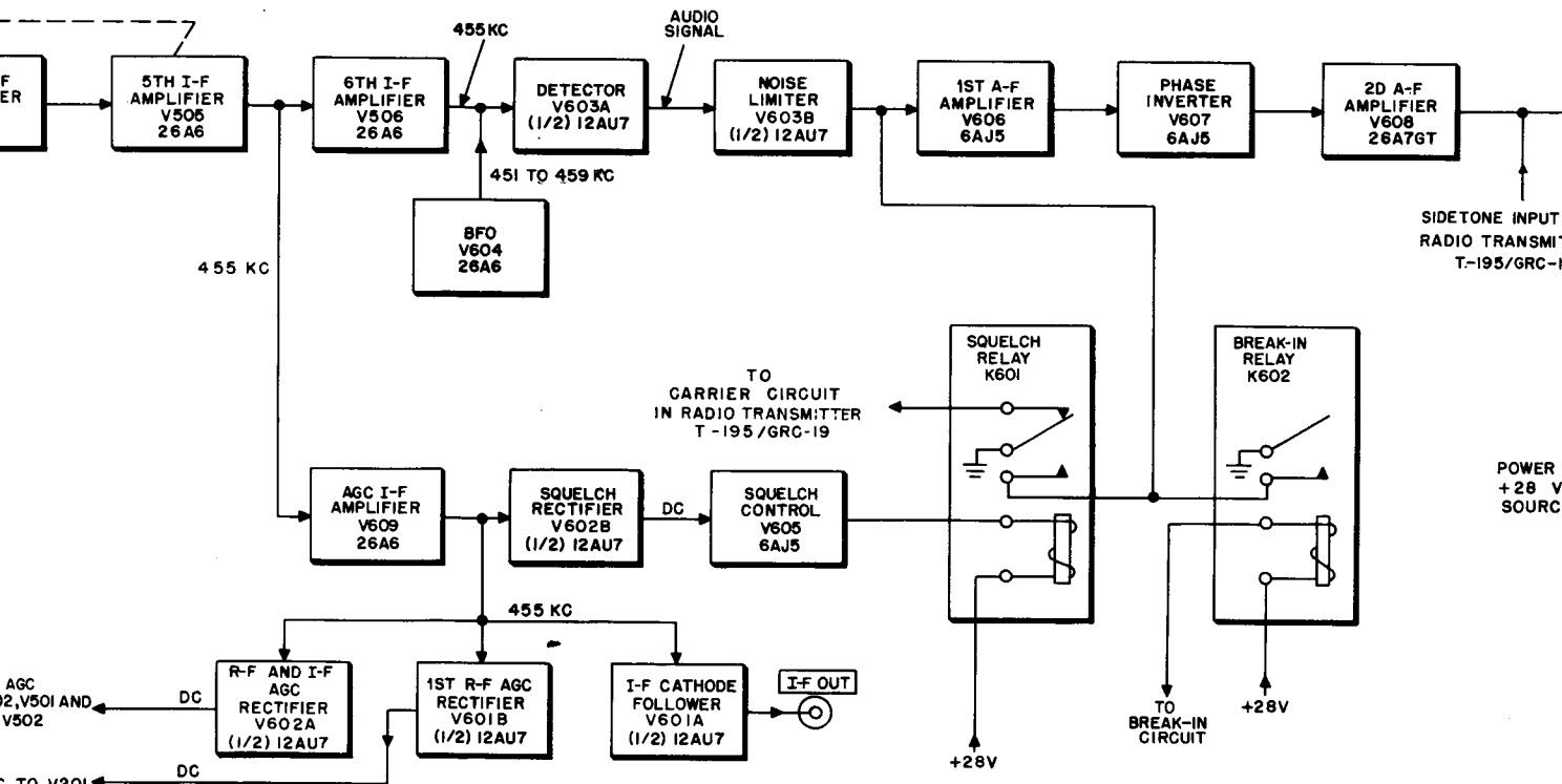
Figure 1. Radio Receiver R-392/URR, block diagram.
