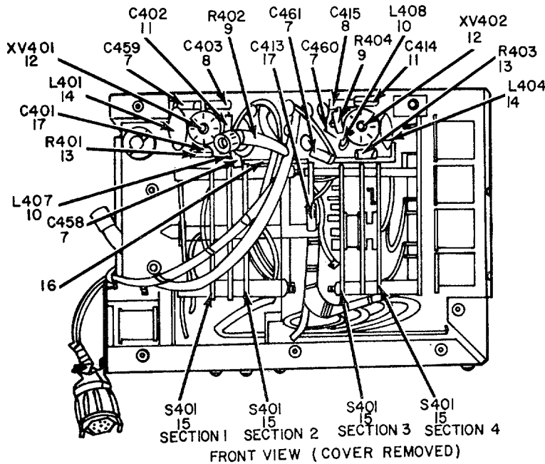
Figure 12. Oscillator, Radio Frequency, Crystal Controlled.
