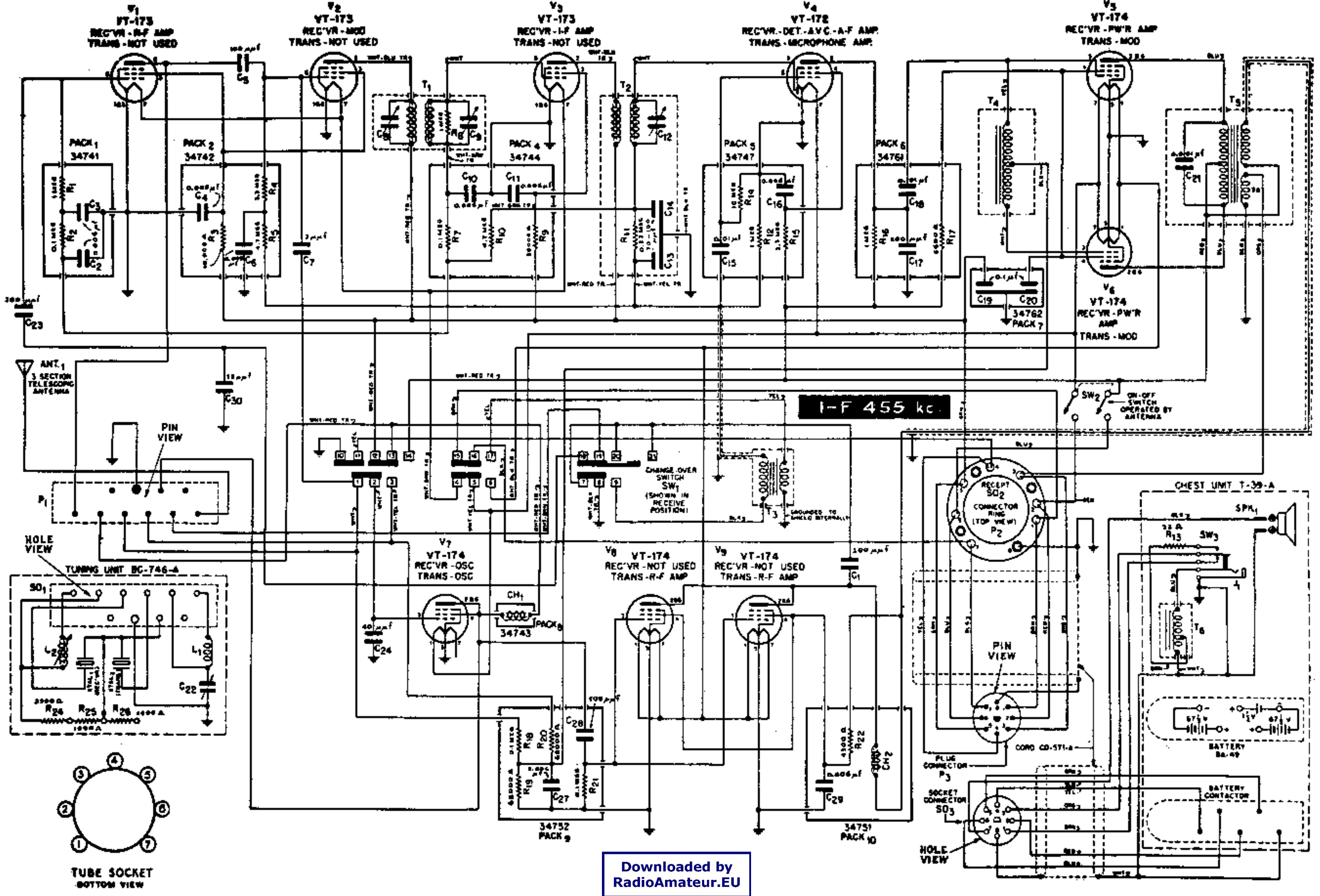
Schematic—BC-745-A (Late) Including Tuning Unit BC-746-A and Chest Unit T-39-A.
