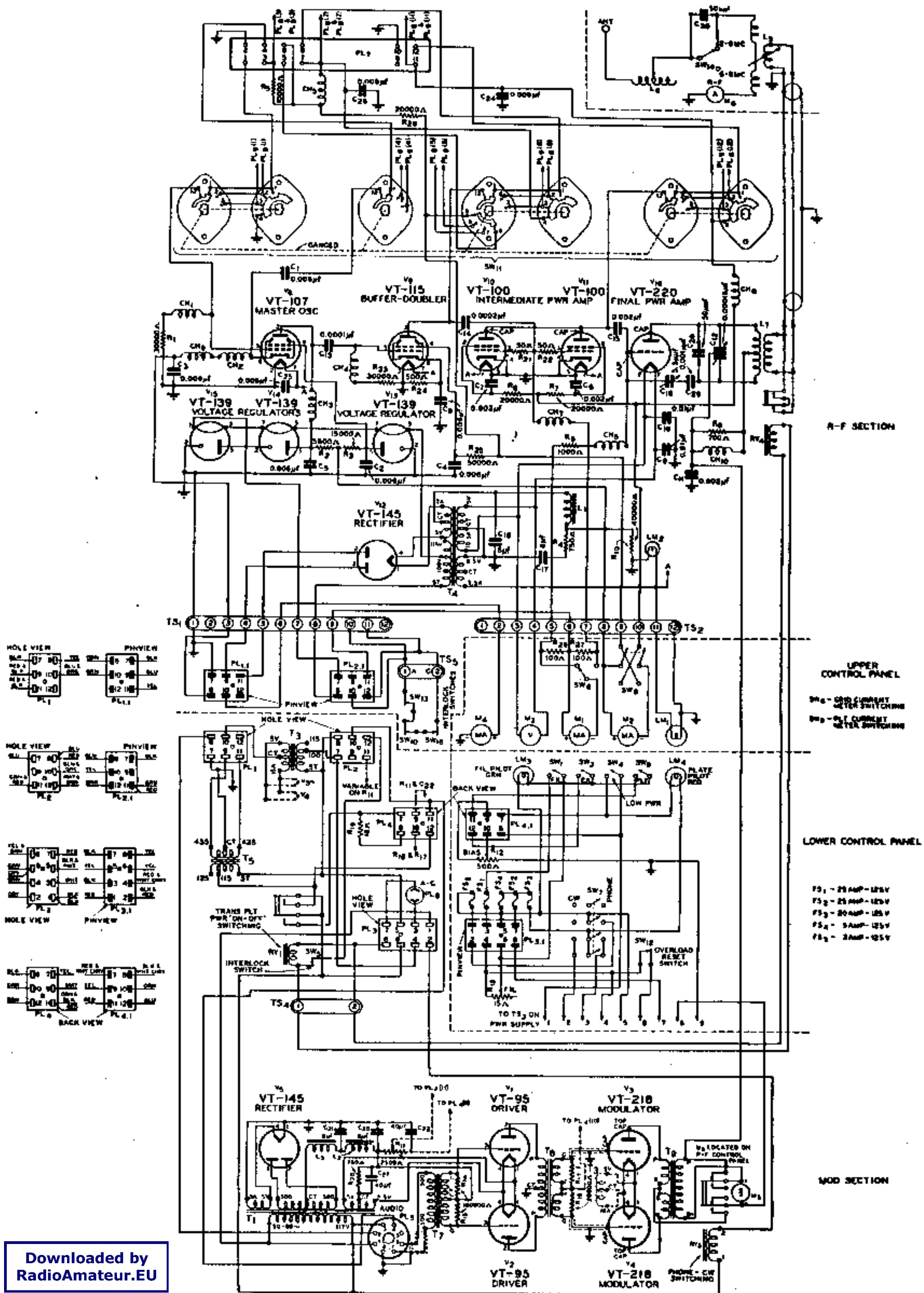
Fig. 9.—Schematic BC-610-D
