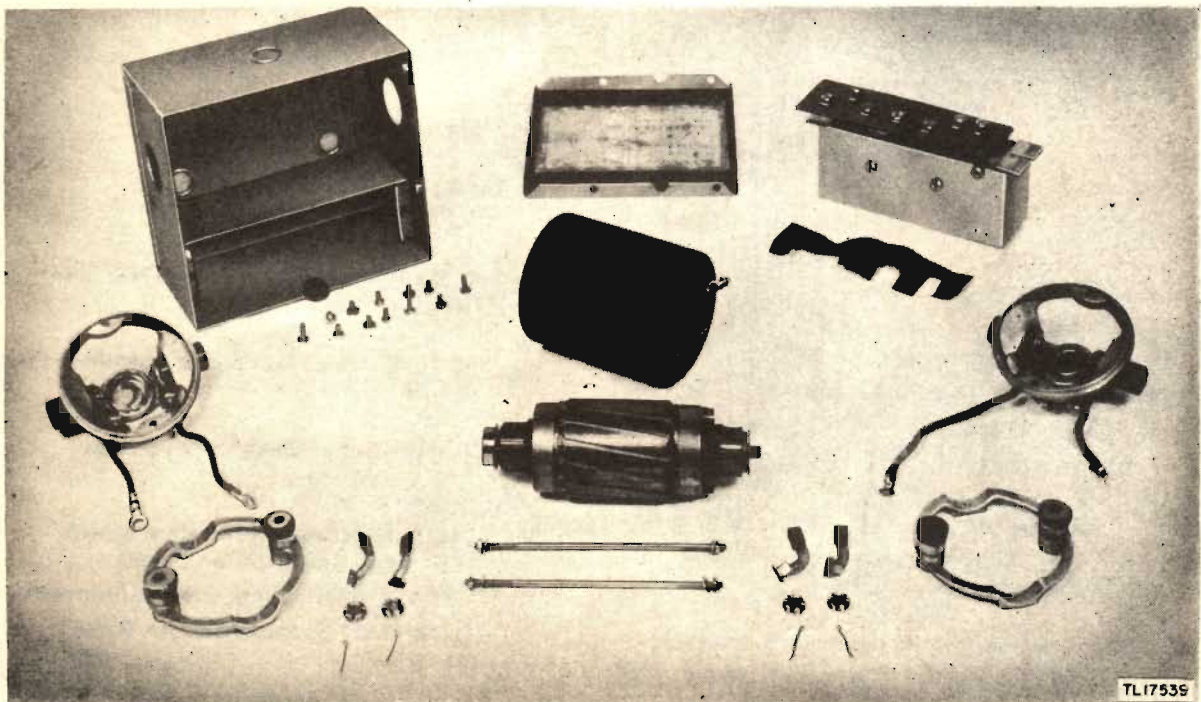
Figure 8. Dynamotor parts.
