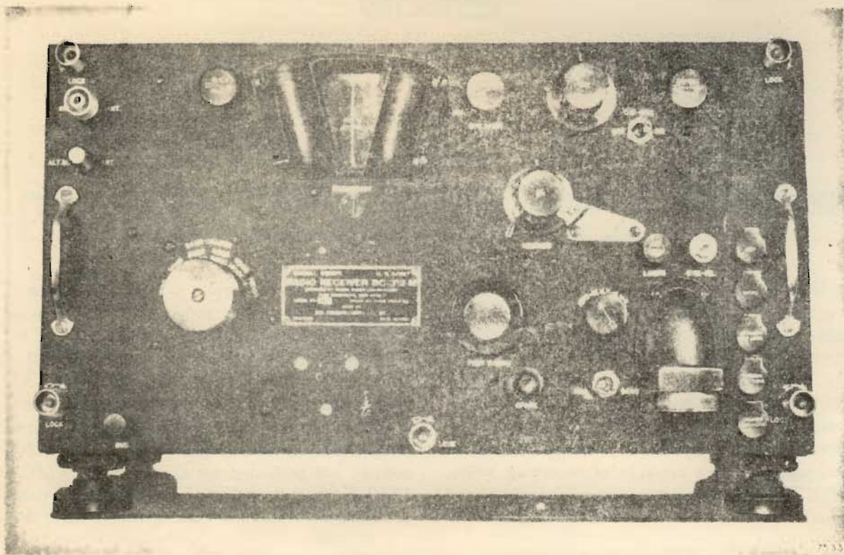
Figure 2. Radio Receiver BC-312-M, front view.
