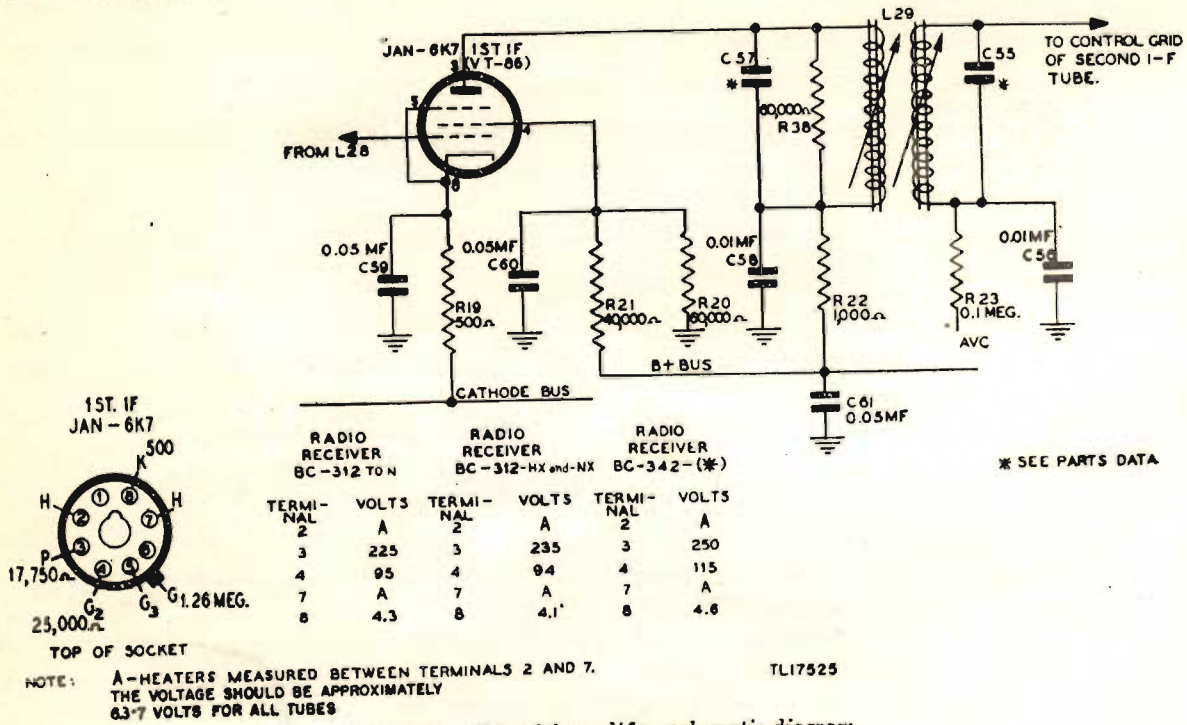
Figure 26. First i-f amplifier, schematic diagram.
