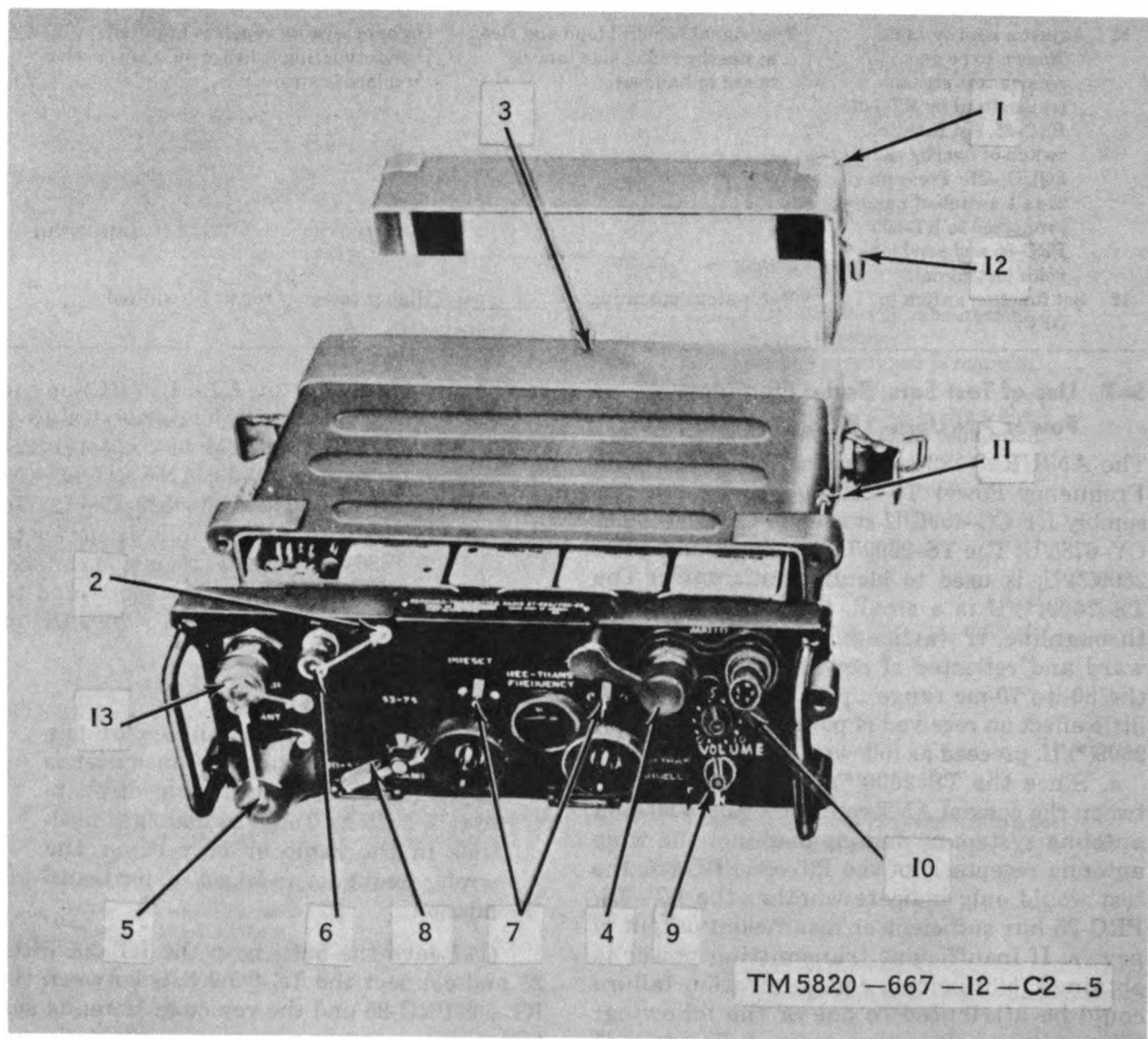
Figure 5-1. Receiver-Transmitter, Radio RT-505/PRC-25, parts.
