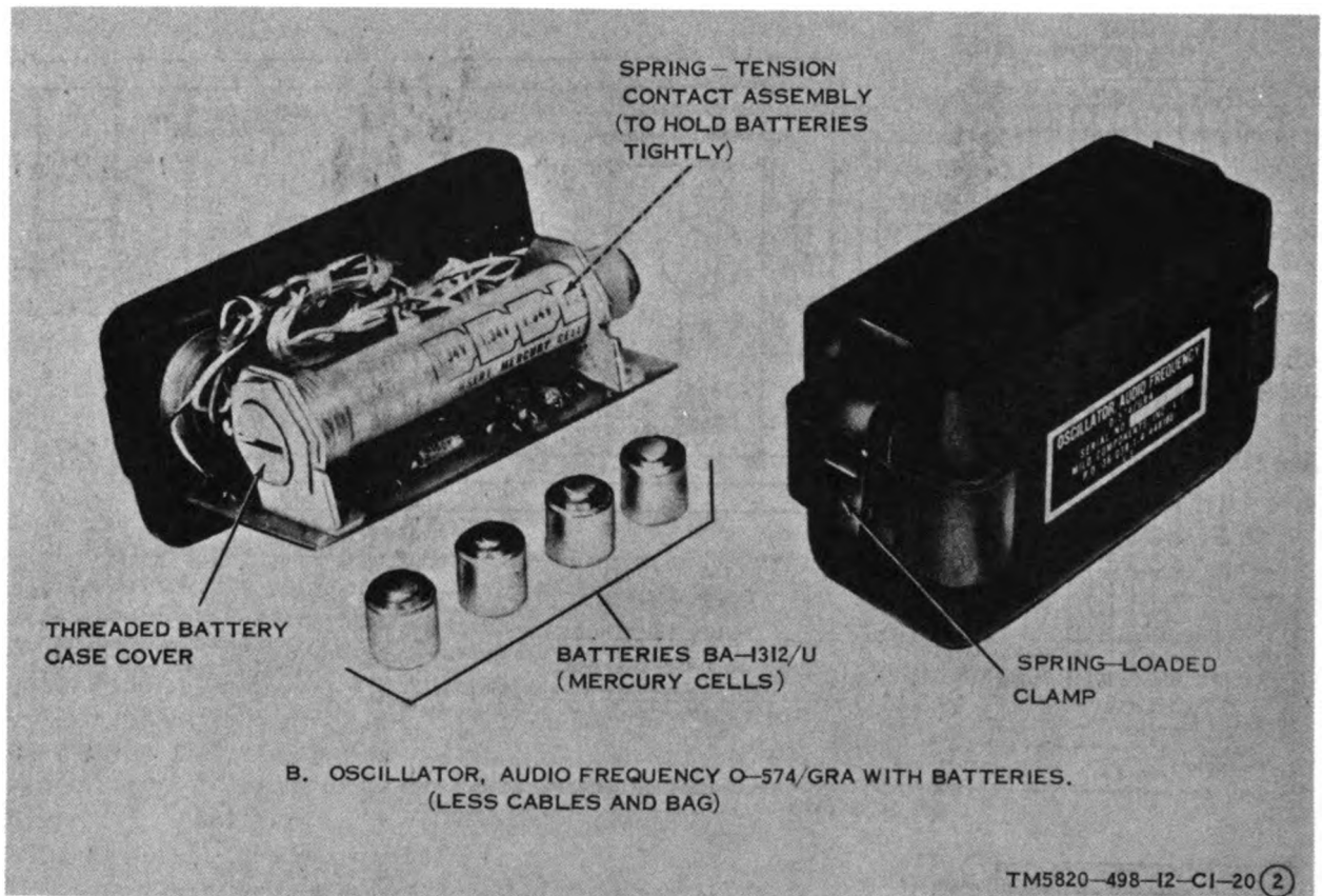
Figure 6-18. Oscillator, Audio Frequency O-574/GRA with Batteries, Dry BA-1312/U.
