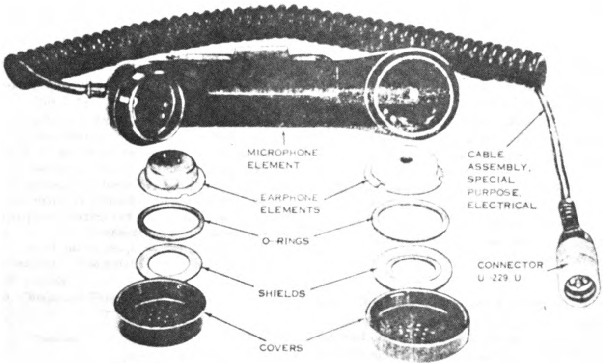
Figure 1-3. Handset H-189/GR, disassembled.
