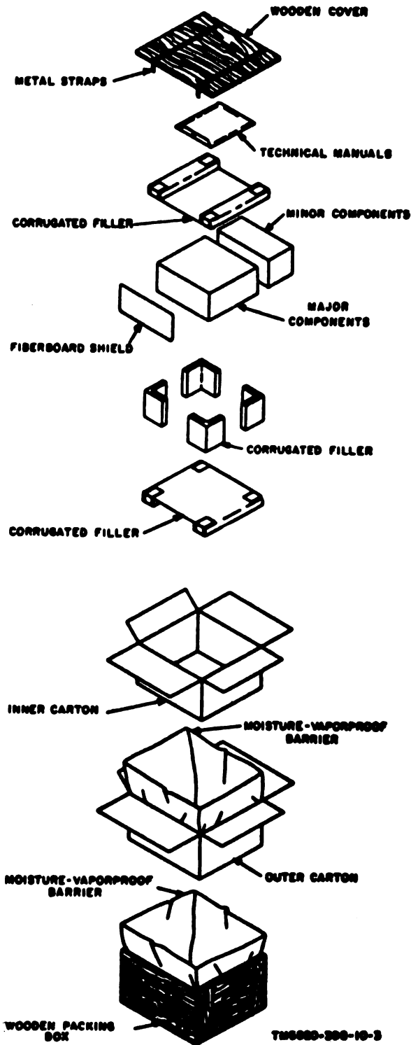
Figure 2-1. Typical packaging.
