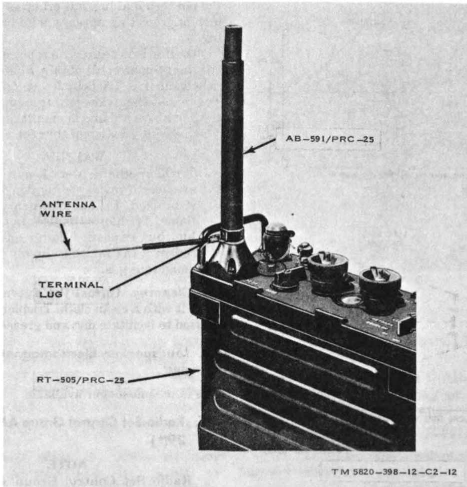
Figure 6-7. Connection of antenna wire of AT-984A/G to RT-841/PRC-77.
