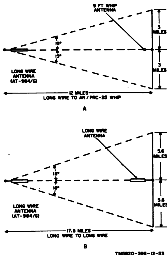
Figures 6-6. AT-984A/G, radiation patterns and siting diagram.
