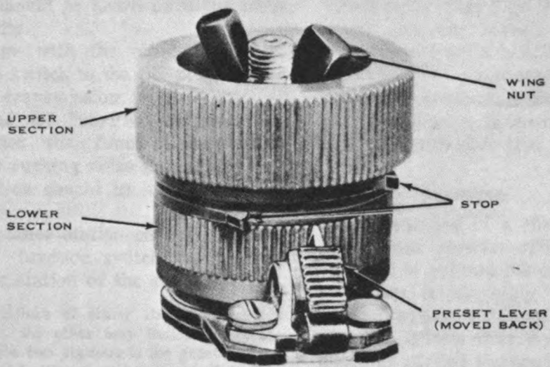
A. TUNING CONTROL; LOWER AND UPPER SECTIONS LIFTED.
