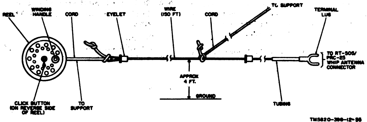
Figure 6-8. Antenna AT-824A/G, installation and parts.
