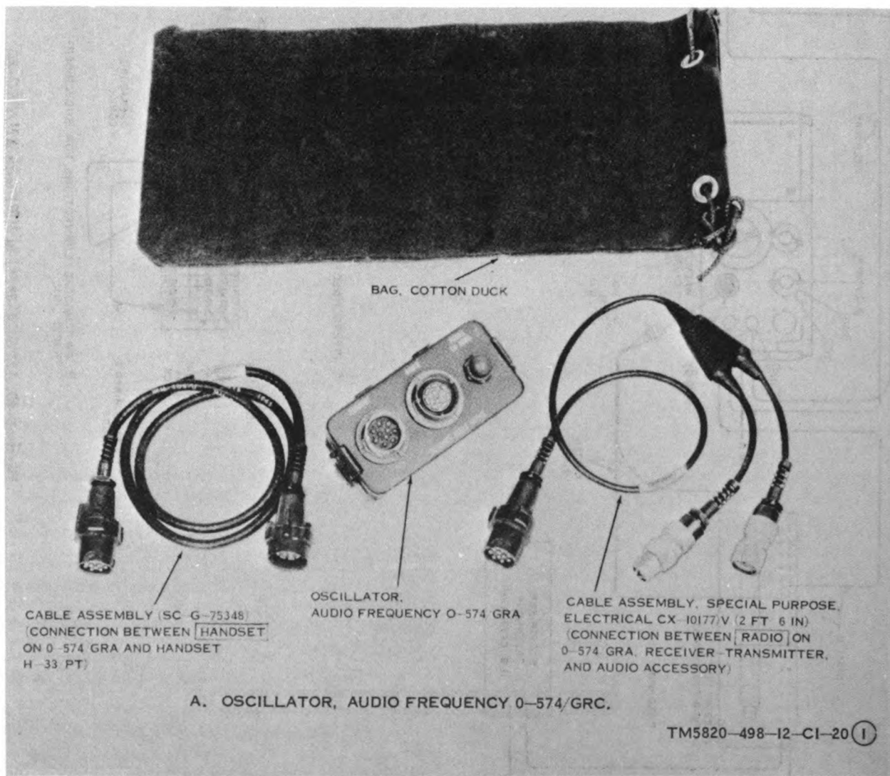
Figure 6-11. Oscillator, Audio Frequency O-574/GRA.
