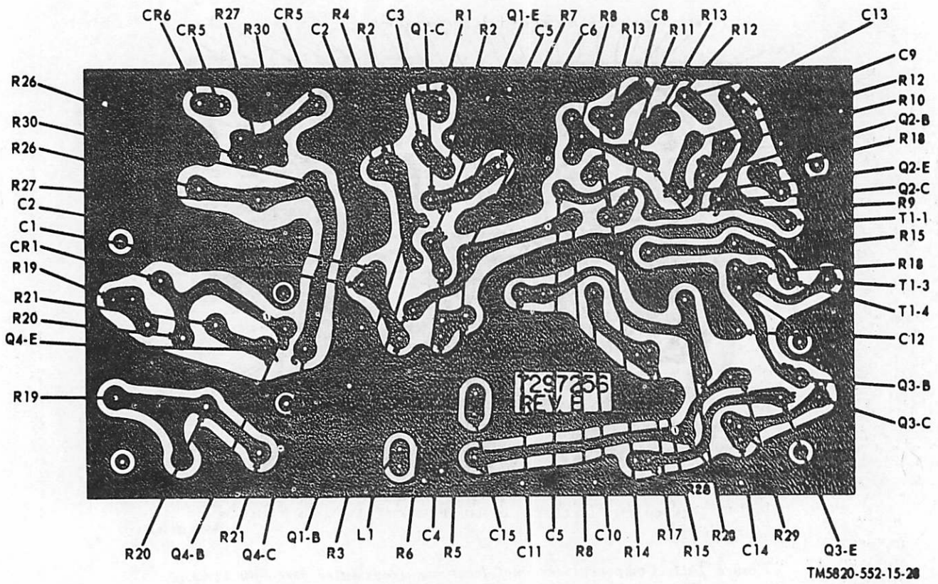
Figure 7-13. Component terminal locations, modulator and battery test assembly A4A2.
