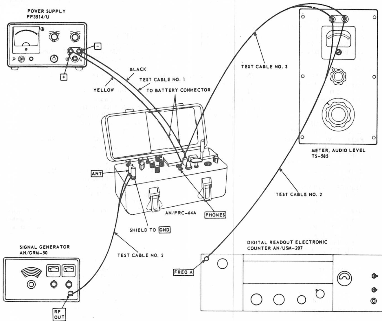
Figure 7-23. Receiver tests.
